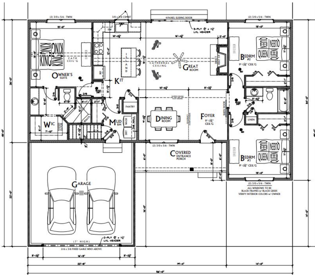
MAIN LEVEL PLAN
